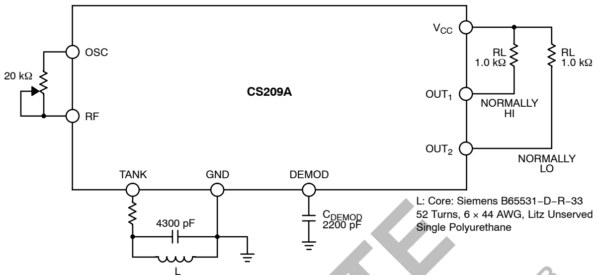
Figure 5. Test and Application Diagram
